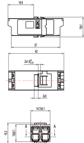
Duplex without flange
