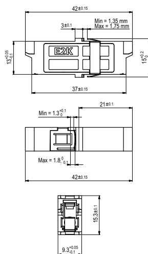
Simplex without flange
