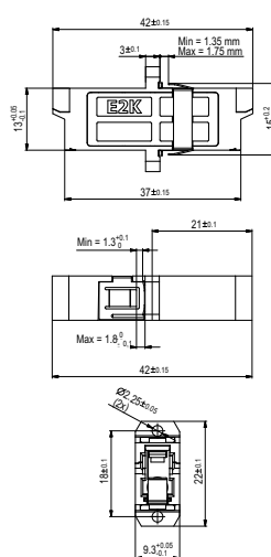
Simplex with flange
