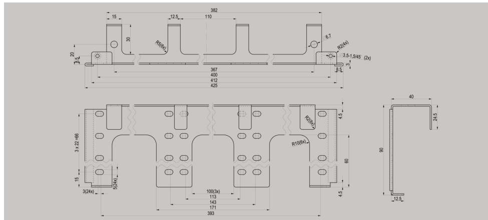
Management bar with labeling plate mounting possibility Management bar with labeling plate mounting possibility, light grey RAL 7035 Management bar with labeling plate set, light grey RAL 7035
