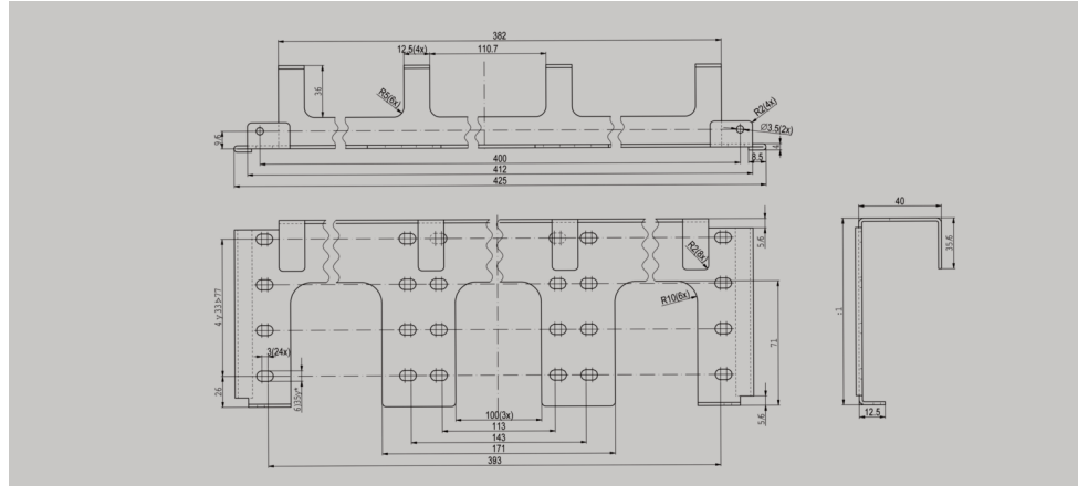
Management bar without labeling plate mounting possibility Management bar without labeling plate mounting possibility, light grey RAL 7035
