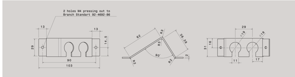
Cable entry plate rechargeable angular
